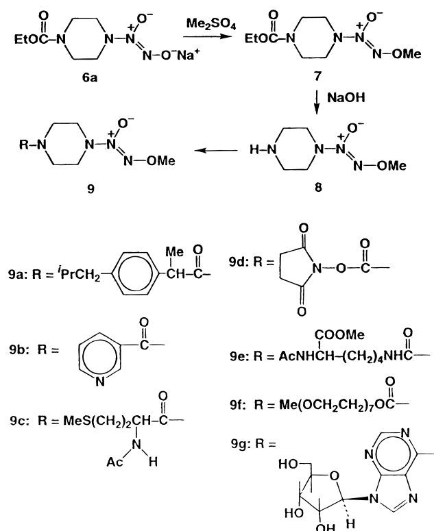
Scheme 2. Synthesis of O 2 -Methylated Piperazine Diazoniumdiolates
