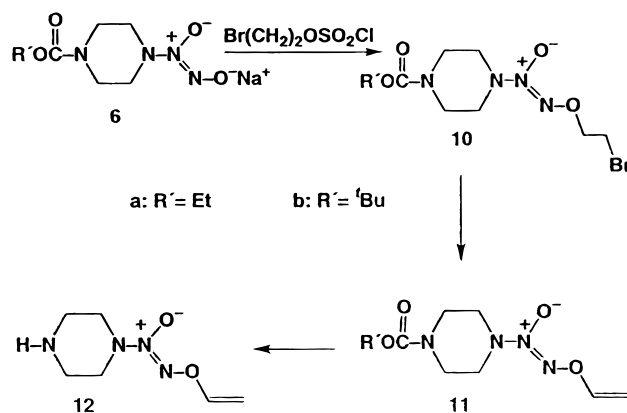
Scheme 3. Synthesis of O 2 -Vinylated Piperazine Diazoniumdiolates
