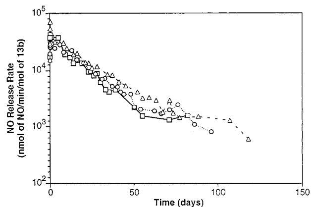
Figure 1. Observed rates of NO generation from 13b at initial concentrations of 20–50 mM at various times after dissolution in 0.1 M phosphate buffer at 37 °C. Individual results for three separate incubations are shown. The pH remained at 7.4 throughout the incubations.
