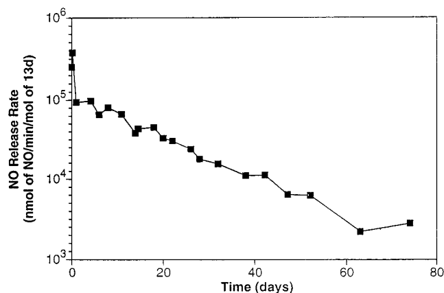
Figure 2. Time course of NO release observed on suspending 10 mg of diazeniumdiolated phospholipid 13d in 2 mL of 0.1 M phosphate buffer (pH 7.4) at 37 °C.
